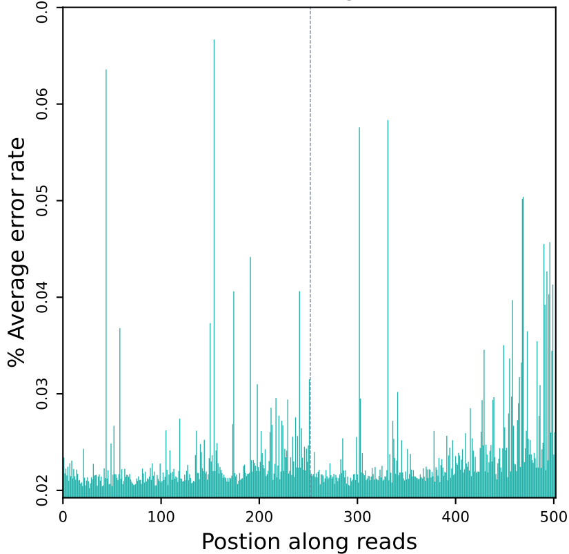
Error rate distribution along reads (R10708)
